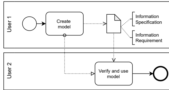
Fig. 3. Minimum BPMN diagram input for the demonstration case
