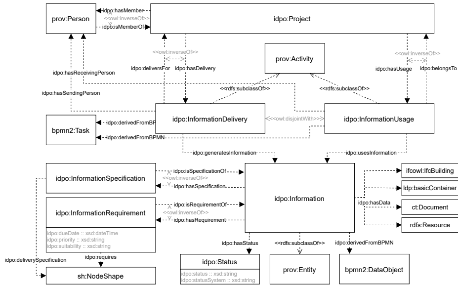
Fig. 2. Overview of the Information Delivery Process Ontology (IDPO)
