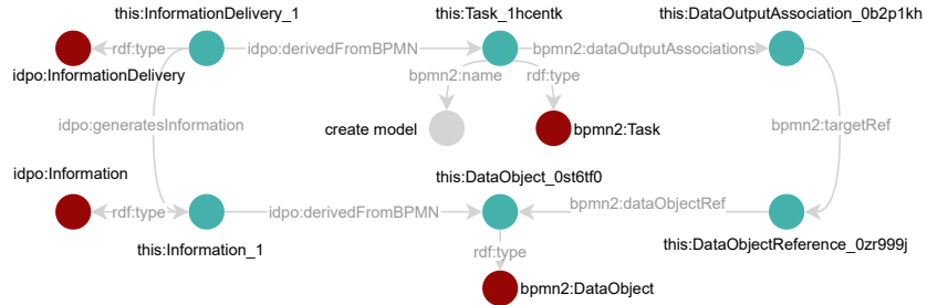
Fig. 4. BPMN to IDPO conversion output
