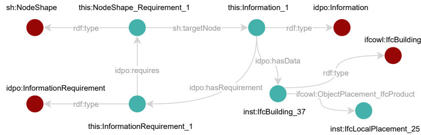
Fig. 5. Applying sh:NodeShape requirements targeting idpo:Information instances
